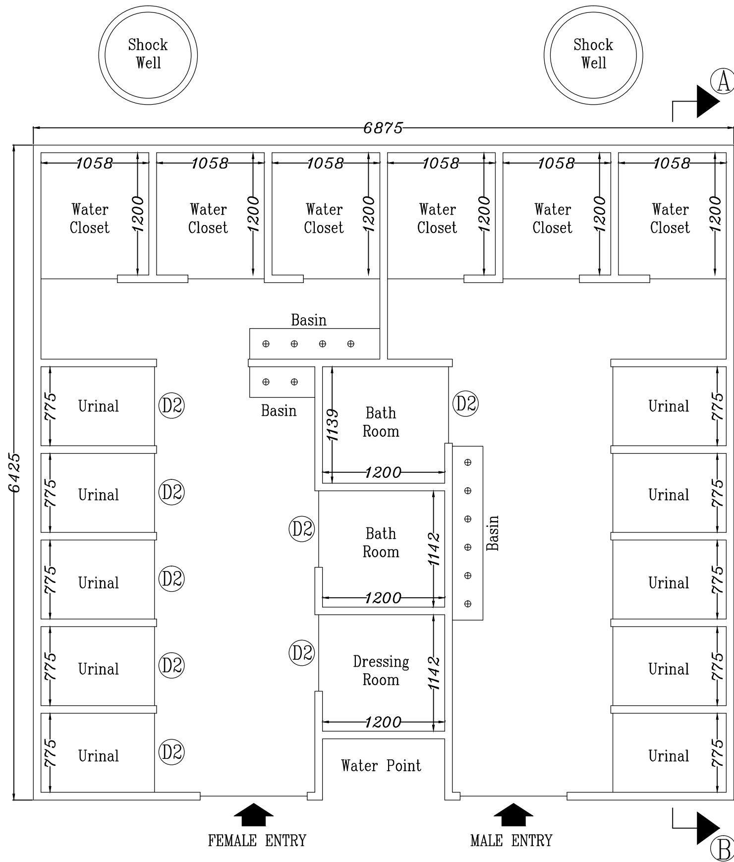
TEMPORARY TOILET BLOCK PLAN AT POUS MELA, 2019
